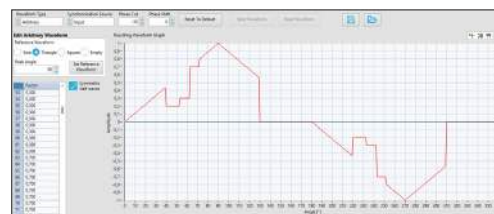
Arbitrary waveform
